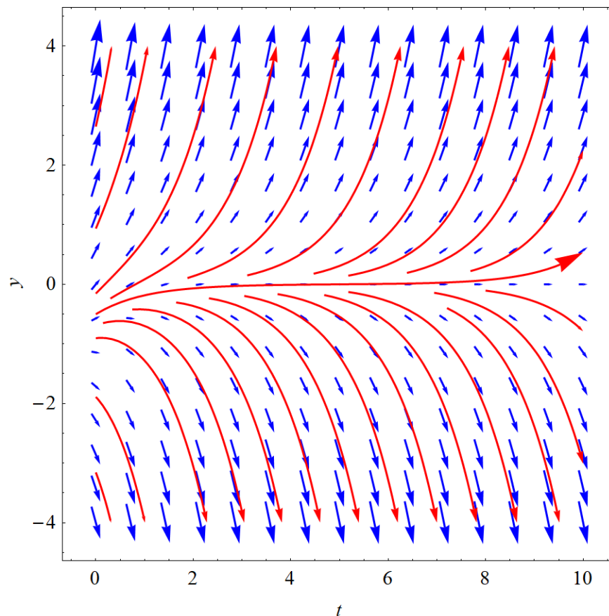
Figure 1: In blue are the direction field vectors and in red are possible solutions to the differential equation, depending what the initial condition is. If the initial condition is below a certain curve in the ty -plane, then the solution diverges to -\infty , and if the initial condition is above this curve, then the solution diverges to \infty .
