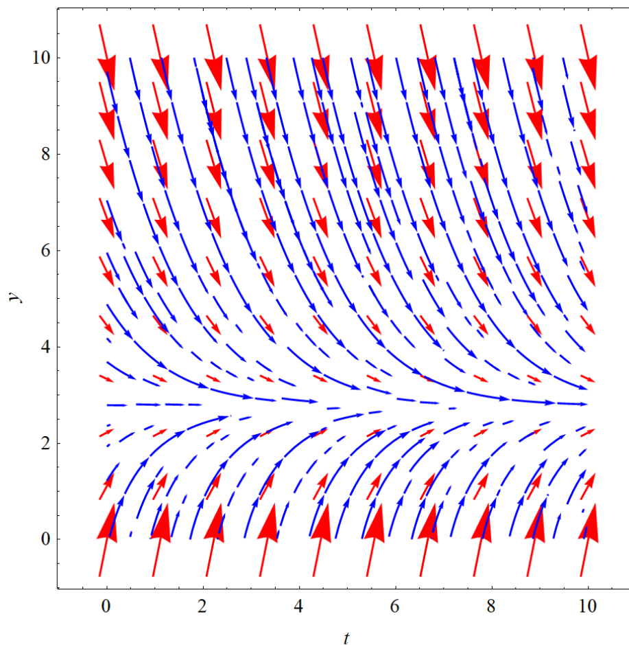
Figure 1: In red are the direction field vectors and in blue are possible solutions to the differential equation, depending what the initial condition is. All solutions appear to converge as t \rightarrow \infty .
