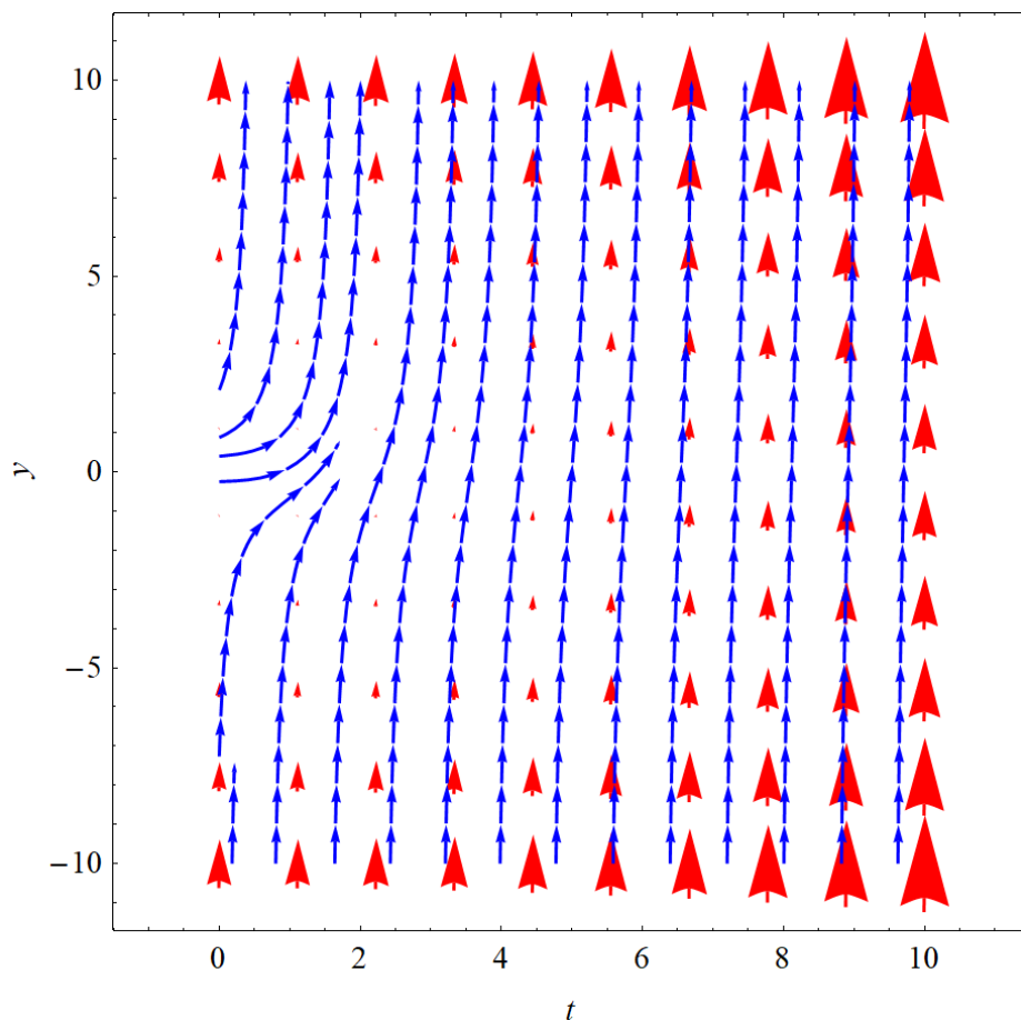
Figure 1: In red are the direction field vectors and in blue are possible solutions to the differential equation, depending what the initial condition is. All solutions appear to diverge as t \rightarrow \infty .
