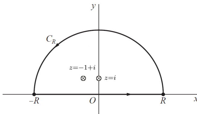
Figure 1: This is Fig. 93 with the singularity at z = -1 + i marked.
