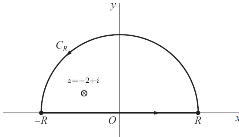
Figure 1: This is Fig. 93 with the singularity at z = -2 + i marked.
