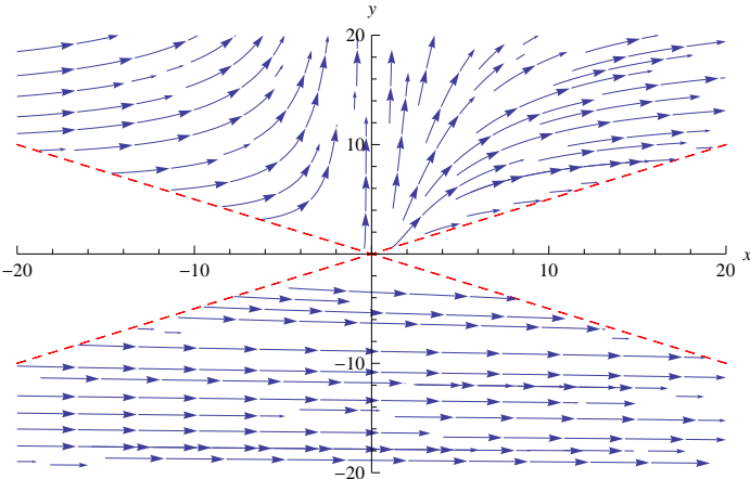
Figure 1: Slope field for \frac{dy}{dx} = \frac{1}{x^2} (2y + \sqrt{4y^2 - x^2})
