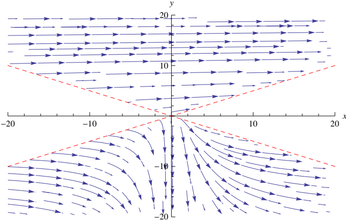
Figure 2: Slope field for \frac{dy}{dx} = \frac{1}{x^2} (2y - \sqrt{4y^2 - x^2})
