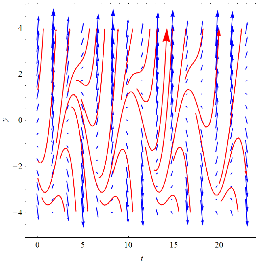
Figure 1: In blue are the direction field vectors and in red are possible solutions to the differential equation, depending what the initial condition is. The solutions appear to diverge from a sinusoidal curve as t \rightarrow \infty . If the initial condition is below the curve, then the solution diverges to -\infty , and if the initial condition is above the curve, then the solution diverges to \infty .
