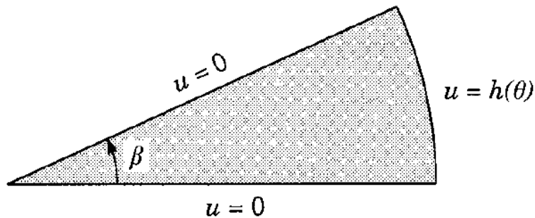
Figure 1: This is Figure 1 on page 173 of the text with the boundary condition along the arc modified to u = h(\theta) . The radius of the wedge is a .
